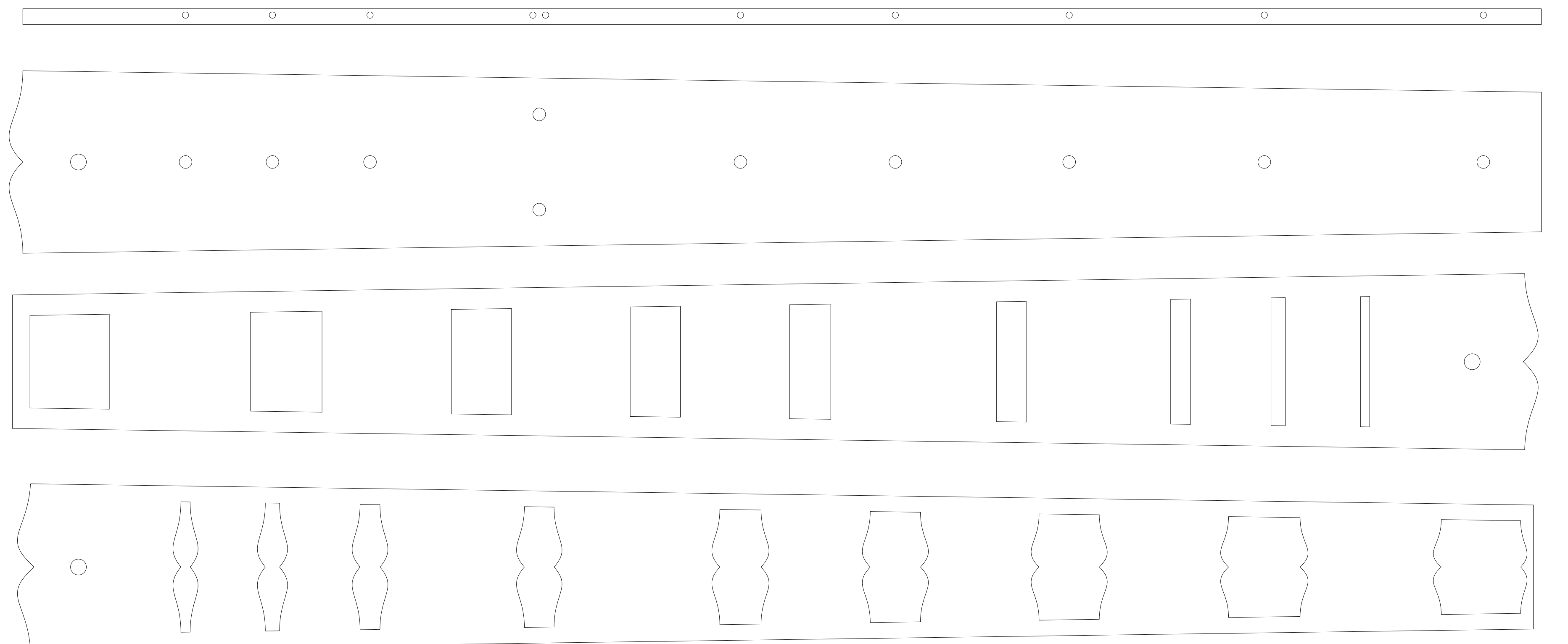
Fretboards
